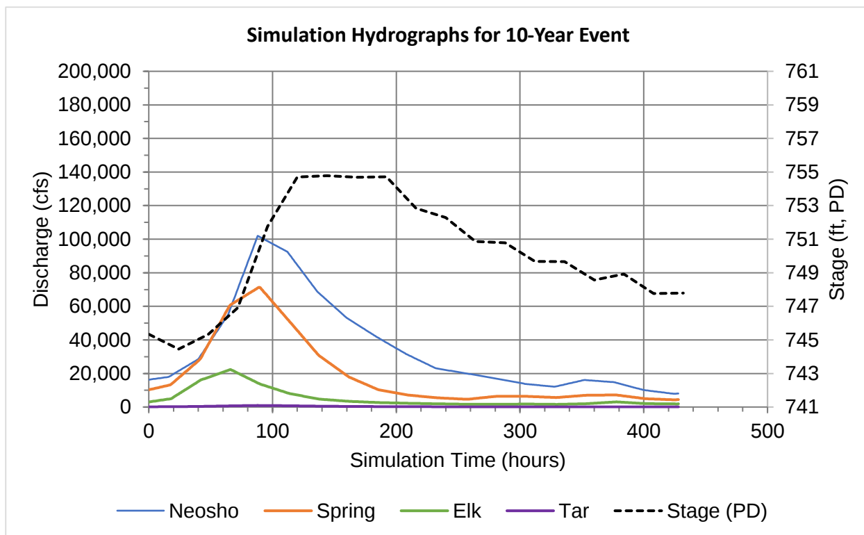
Figure 3. Inflow and stage hydrographs for the 10-year return interval event.
