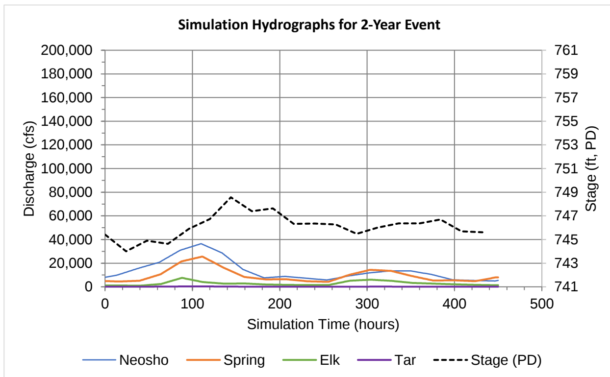
Figure 5. Inflow and stage hydrographs for the 2-year return interval event.
