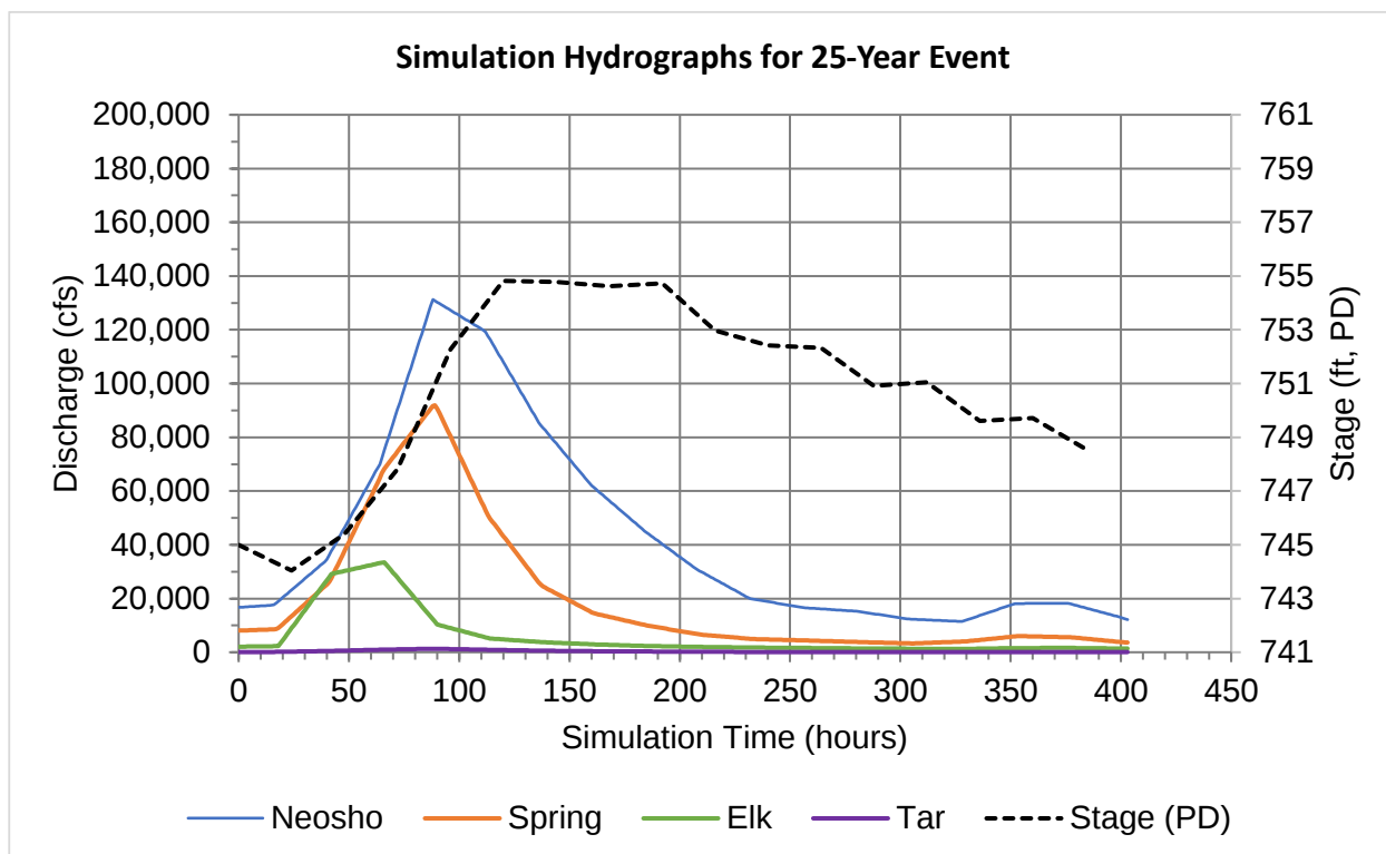
Figure 2. Inflow and stage hydrographs for the 25-year return interval event.
