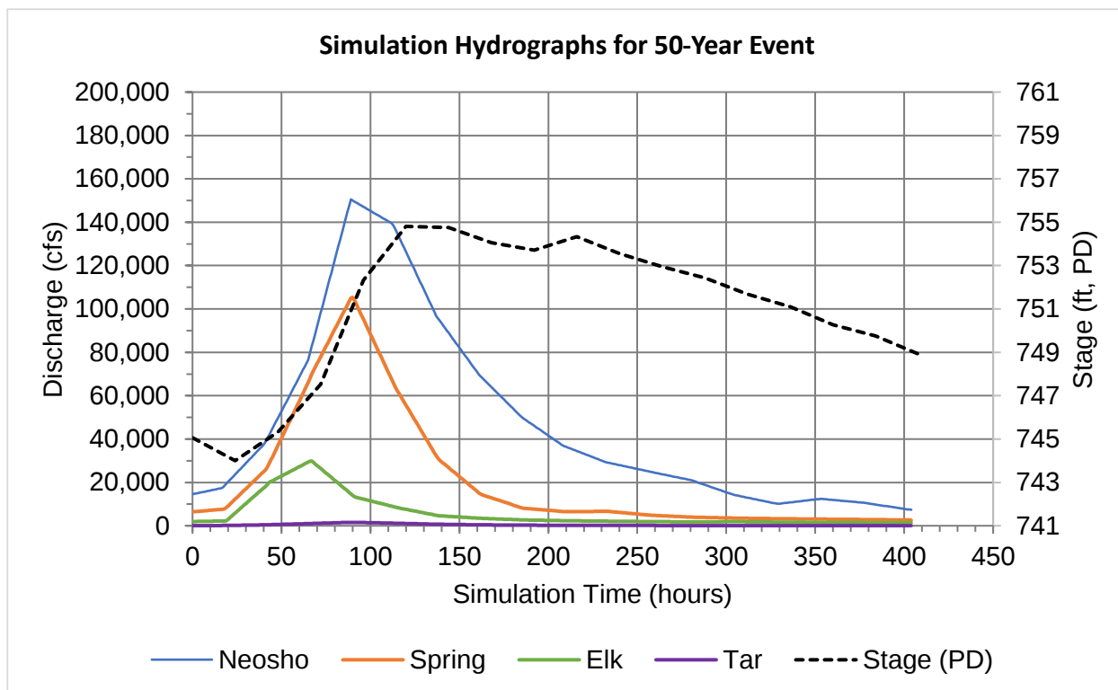
Figure 1. Inflow and stage hydrographs for the 50-year return interval event.
