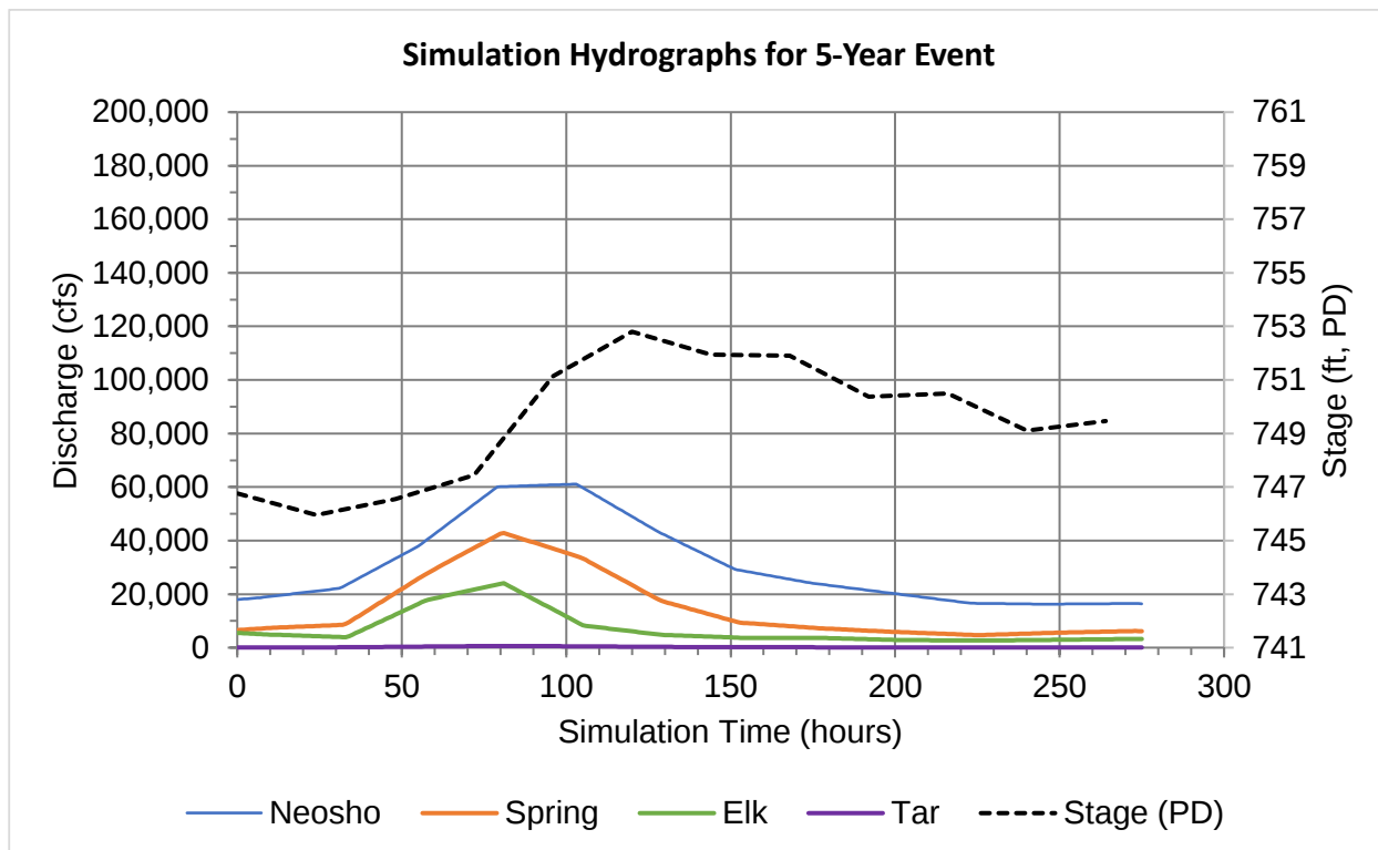
Figure 4. Inflow and stage hydrographs for the 5-year return interval event.
